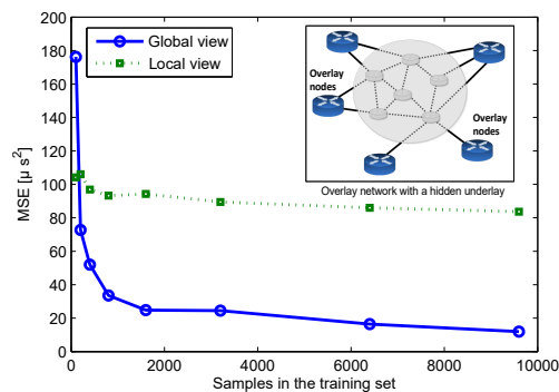
Figure 2: Prediction error (Mean Square Error) as a function of the size of the training set in an overlay-underlay scenario, both for global set and local view.
